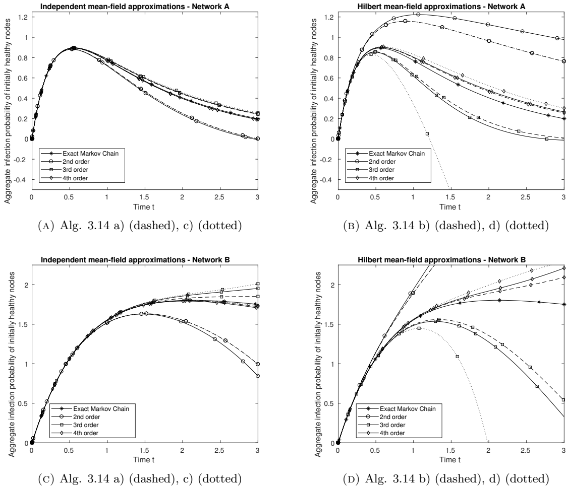
FIGURE 5. Aggregate infection probability of initially healthy nodes. Solid lines represent naive single split approximations; dashed lines correspond to the results of Algorithm 3.14 ( \alpha = 0.5 ) under a single split; dotted lines represent the results of Algorithm 3.14 ( \alpha = 0.5 ) under an equal split.
