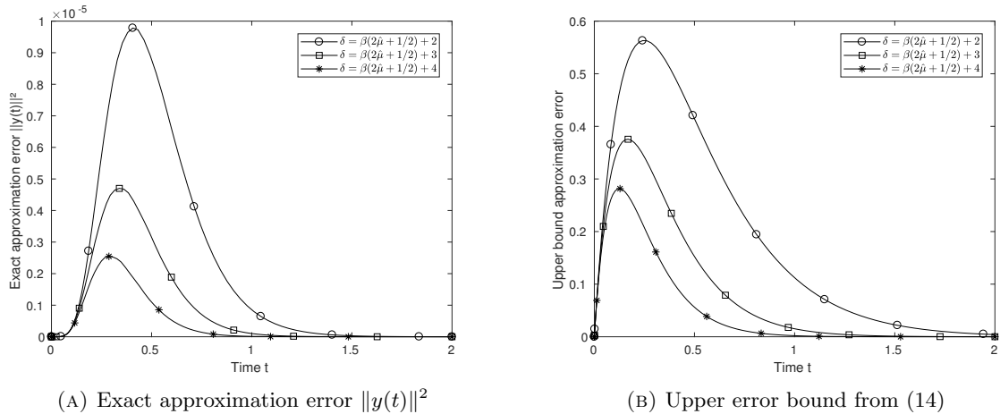
FIGURE 3. Exact approximation error and upper bound for different values of the curing rate \delta and fixed \beta = 1/2 in the regular network A (given in Figure 1) with initial state V(0) = (1, 0, 0, 0, 0, 0)^\top .
