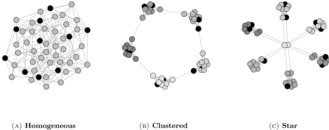
FIGURE 7. Infection scenario: The black nodes (3,5,13,15,23,25,33,35,43,45) are initially infected.
